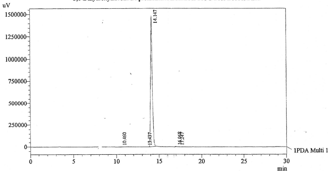
Chromatogram 3,6-Dihydroxyflavone D:\promonence\Data\2013\AUG-2013\100813D.lcd
